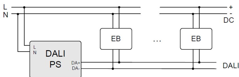
wiring diagram
